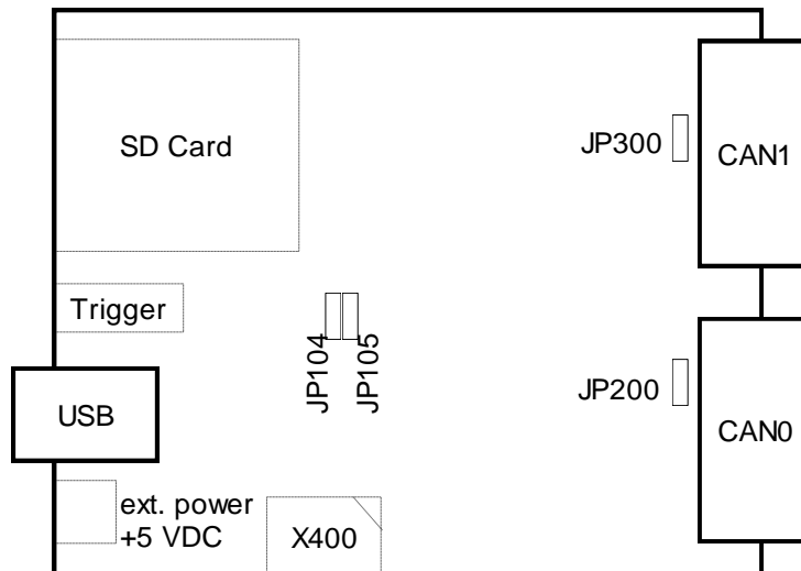
Figure 8: Position of expansion plug and jumpers on USB-CANmodul2
