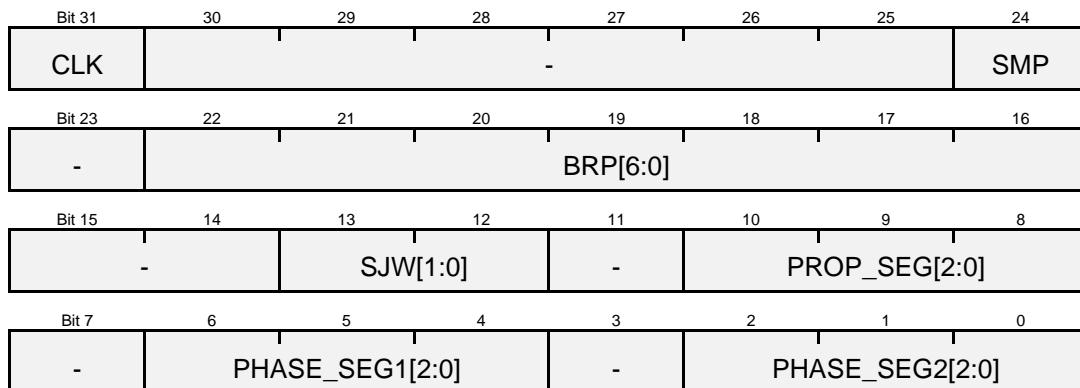
Figure 40: Structure of baud rate register dwBaudrate of third generation modules
