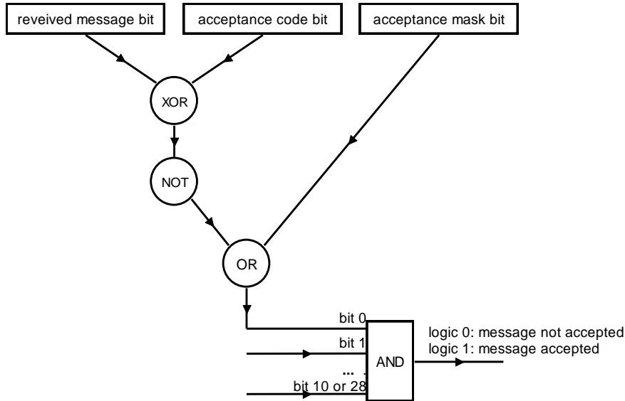
Figure 45: CAN message filter mechanism used within the USB-CANmodul
