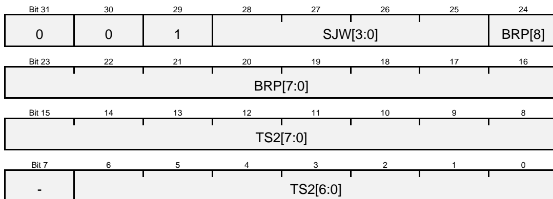
Figure 44: Structure of baud rate register dwBaudrate for fourth generation modules Rev.02
