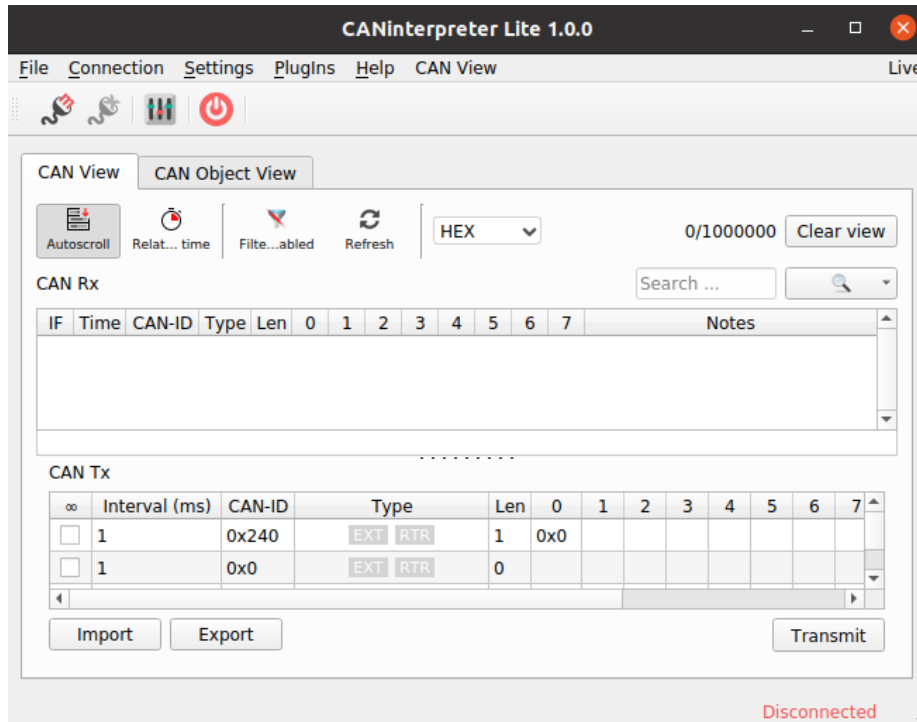
Figure 56: Main window of the CANinterpreter Lite
