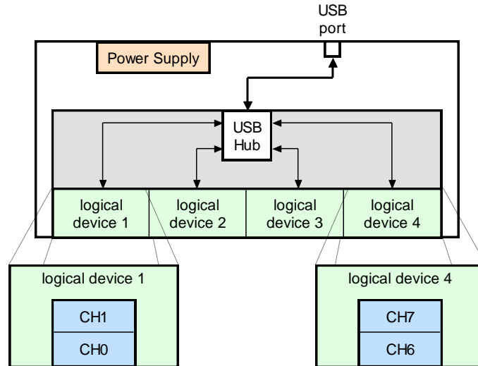
Figure 9: Internal structure of the USB-CANmodul8
