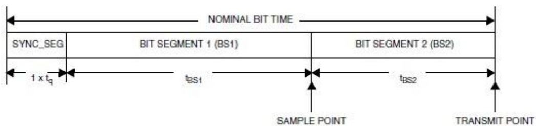
Figure 43: General structure of one bit on the CAN-bus (source: STM32F205xx manual)
