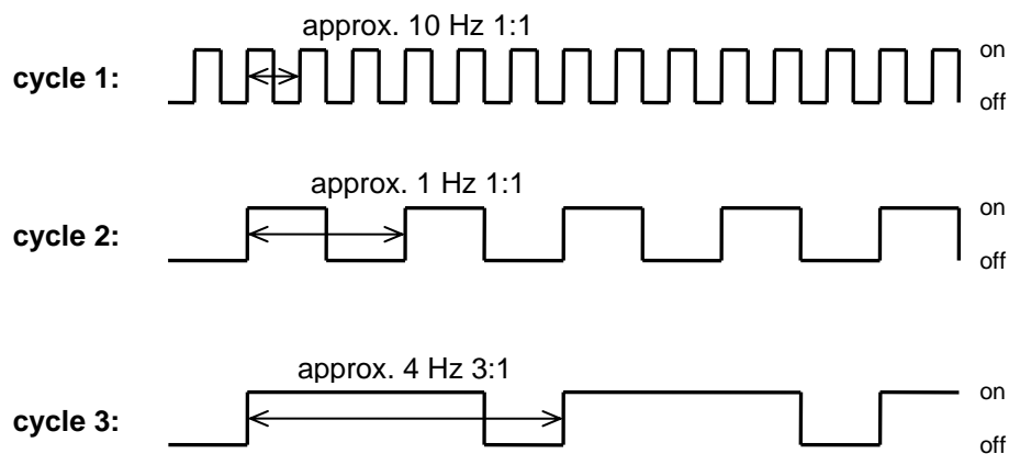
Figure 20: Blink cycles of the state LED
