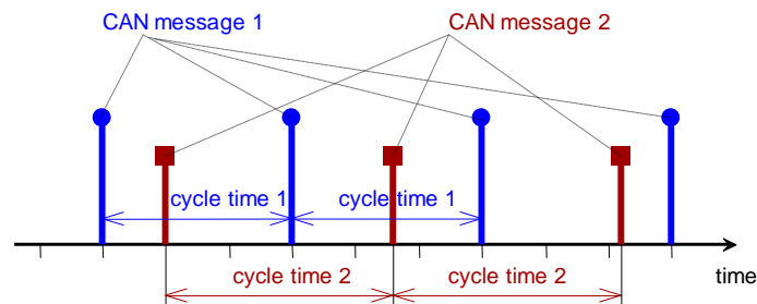
Figure 35: Example for parallel mode of cyclic CAN messages
