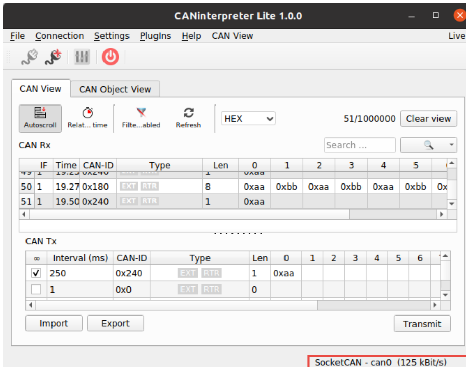
Figure 59: CANinterpreter Lite connected to SocketCAN interface
