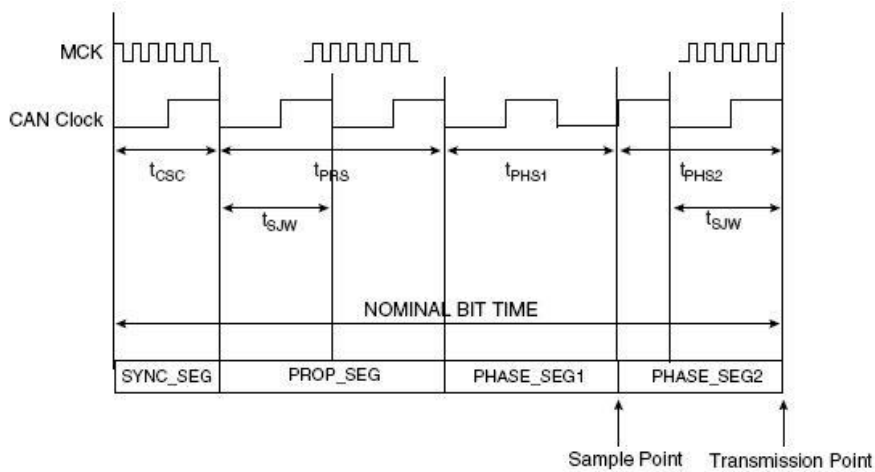
Figure 41: General structure of one bit on the CAN-bus (source: Atmel AT91SAM7A3 manual)
