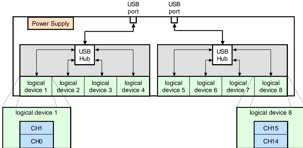
Figure 13: Internal structure of the USB-CANmodul16
