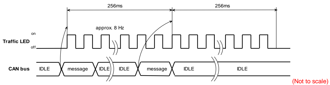
Figure 19: Traffic LED after more CAN messages on CAN bus
