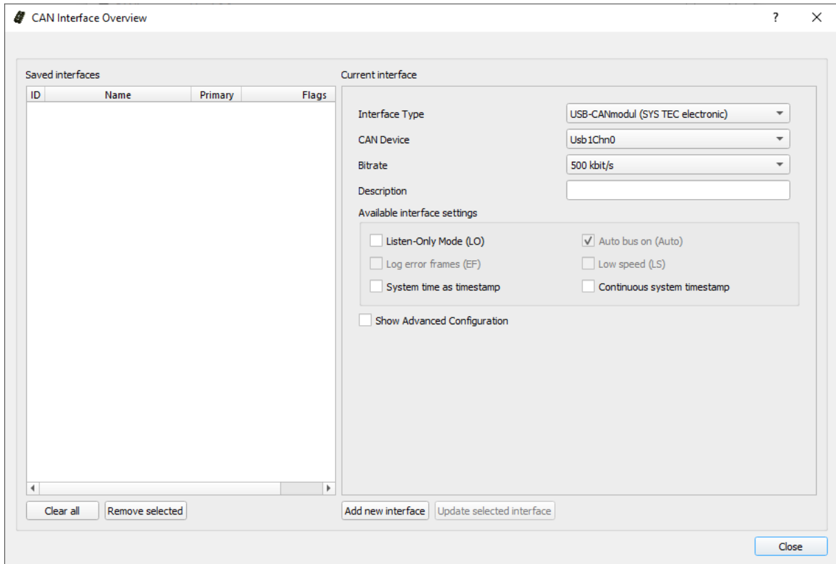
Figure 27: Dialog box for CAN interface Overview in CANinterpreter Lite
