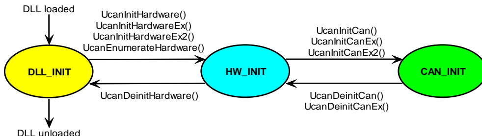
Figure 34: Software State Diagram
