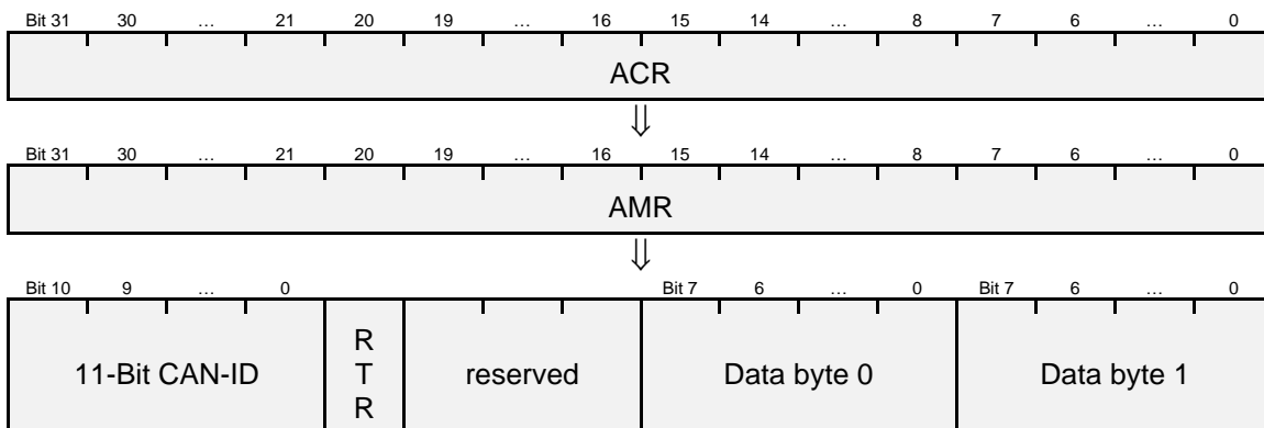
Figure 46: CAN message filter corresponding bits for 11-bit CAN-ID
