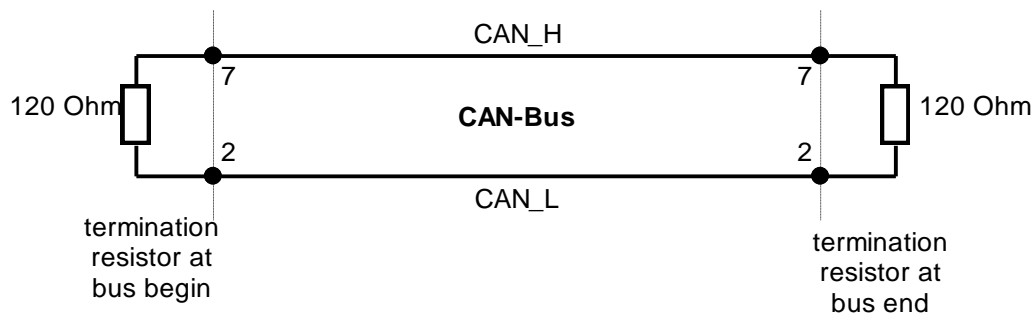
Figure 16: Termination resistors on CAN bus
