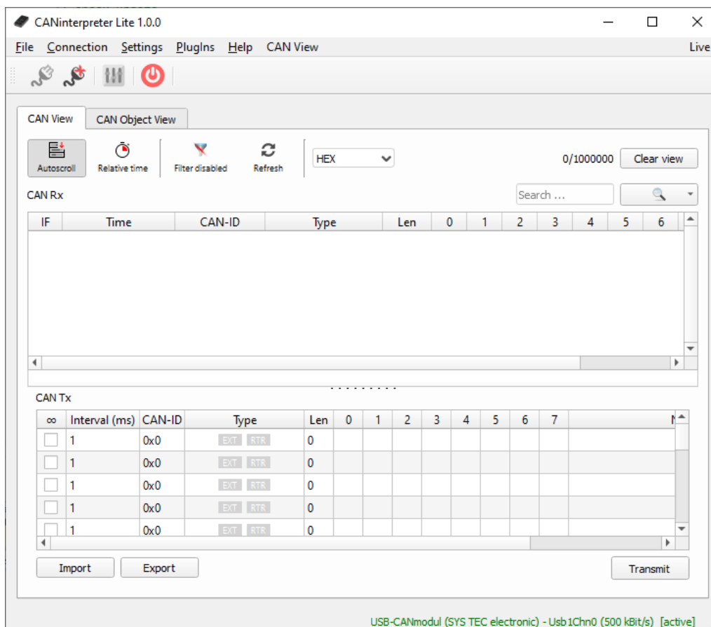
Figure 28: CANinterpreter Lite main window (connected)
