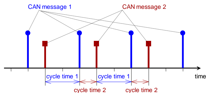
Figure 36: Example for Sequential mode of cyclic CAN messages
