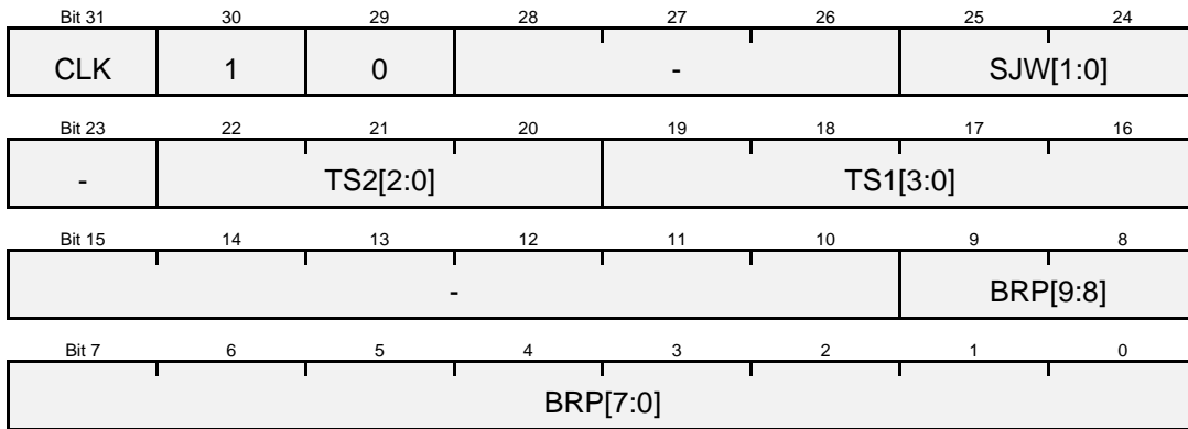
Figure 42: Structure of baud rate register dwBaudrate for fourth generation modules Rev.01
