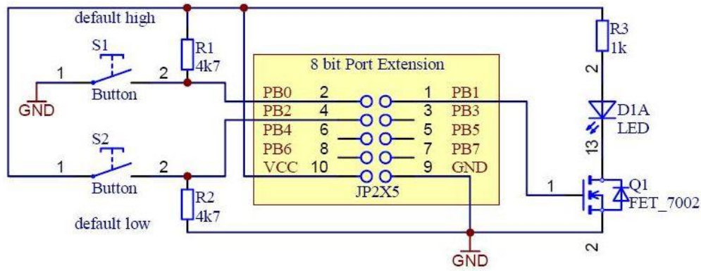
Figure 17: Simple example circuit for Expansion Port
