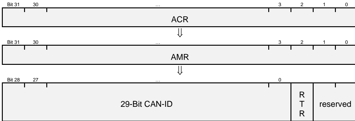
Figure 47: CAN message filter corresponding bits for 29-bit CAN-ID
