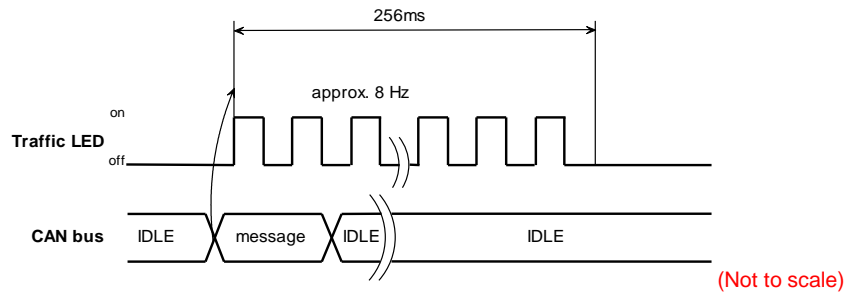
Figure 18: Traffic LED after one CAN message on CAN bus
