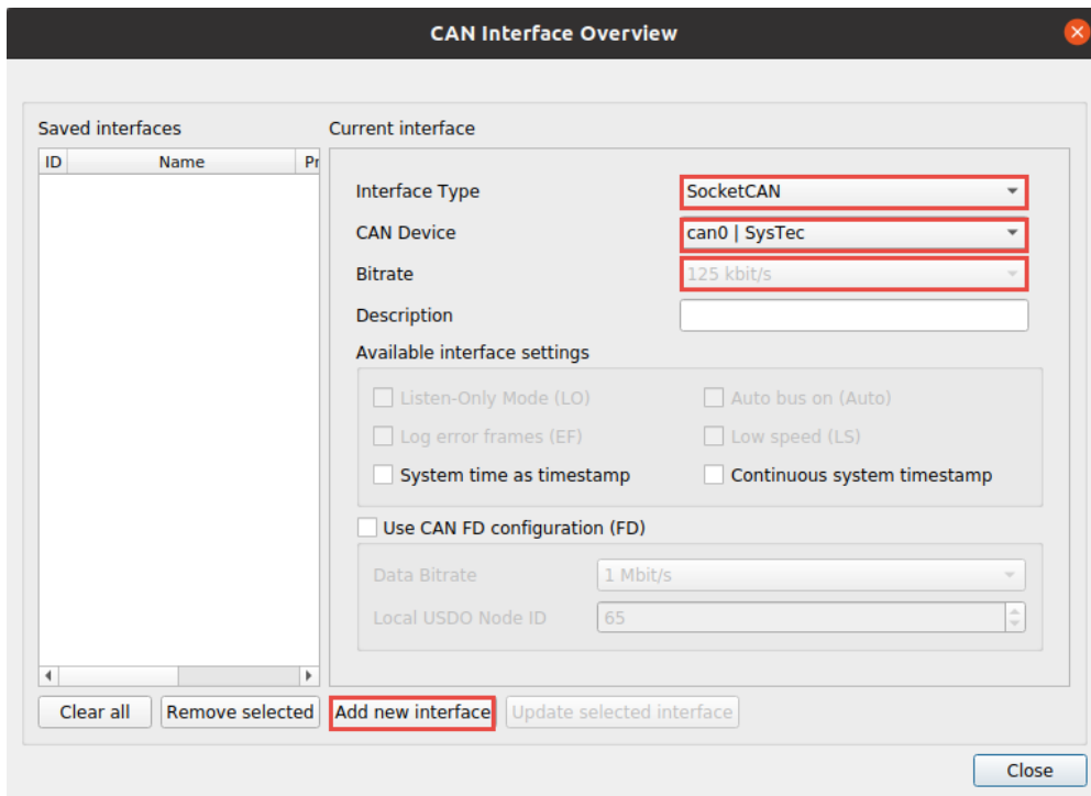
Figure 57: CAN Interface Overview dialog
